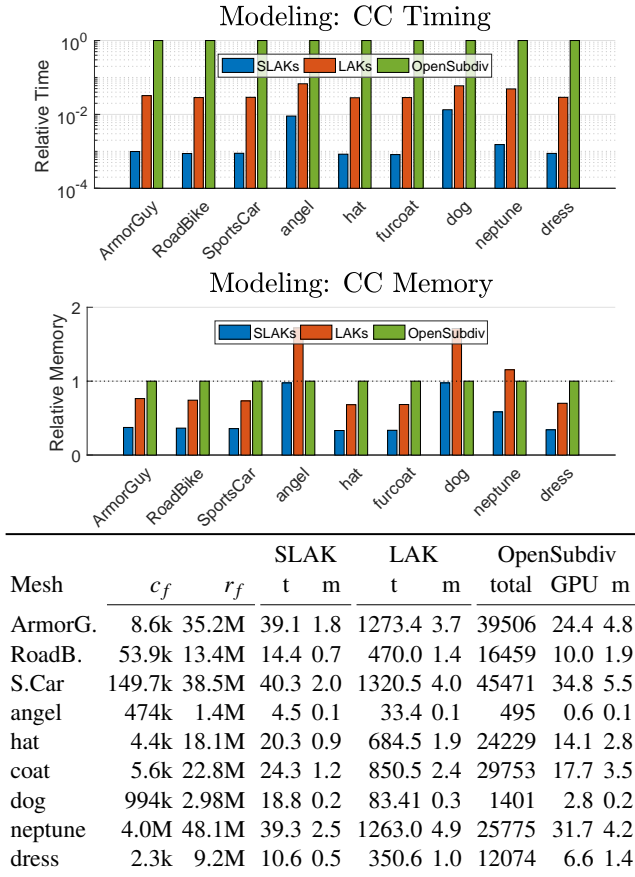
Figure 7: Catmull-Clark subdivision time in ms after a topology changing operation was applied to the mesh. SLAK and LAK relative to OpenSubdiv and relative memory requirements (in GB). Details are given in the table. The number of control mesh faces c_f and the number of refined mesh faces r_f are provided as well.
