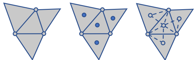
Figure 12: After inserting the new vertices (blue), each triangle contributes three new triangles to the refined mesh by connecting its vertices to their left and right neighboring new vertices.
